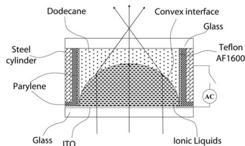
Fig. 1 Schematic cross section of an IL-based EVFLL.
