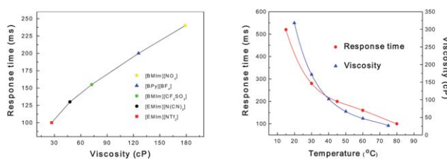
Fig. 5 Response times of five IL-based EVFLL with different viscosities (left) and [EMIm][ClO 4 ]-based EVFLL at variable temperature (right).
