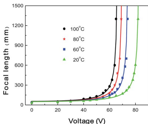
Fig. 4 Change of focal length of EMImClO 4 -based EVFLL with applied voltage at variable temperature. The solid lines are theoretical curves.
