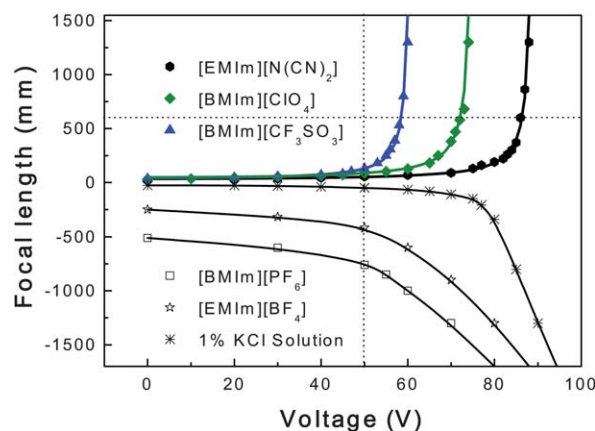
Fig. 3 Change of focal length of five typical ILs and saline-based EVFLL with applied voltage. The solid lines are theoretical curves.
