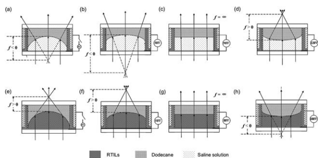
Fig. 2 The curvature of the meniscus of a saline-based EVFLL under 0, 50, 90, 120 V (a–d) and that of an IL-based EVFLL under 0, 50, 80, 100 V (e–h).
